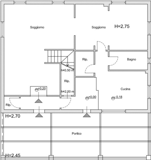
Piano Terra
